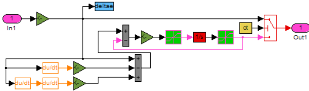
Fig. 11. Matlab/Simulink model of “Forming subsystem for vector deltae (r=2)”
