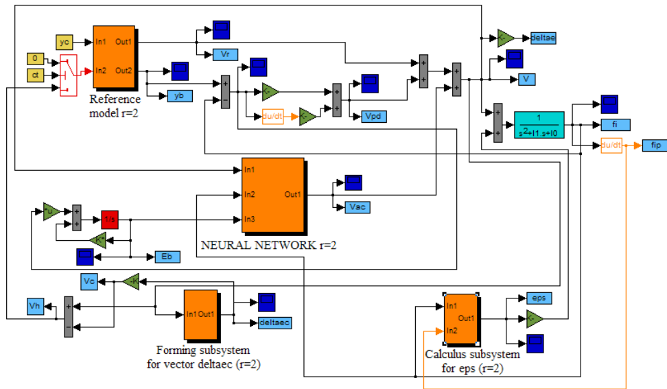
Fig. 8. Matlab/Simulink model for the structure from fig.6
