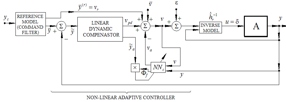
Fig. 3. Automat control system with non-linear adaptive controller
