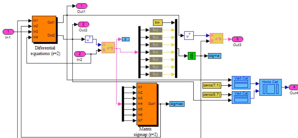
Fig. 9. Matlab/Simulink model for “NEURAL NETWORK r=2 ”
