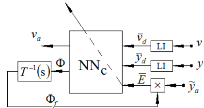
Fig. 5. Block diagram of the adaptive subsystem from din fig. 3
