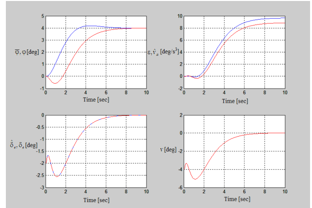
Fig. 13. Time characteristics in the case of linear actuator’s use
