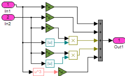
Fig. 12. Matlab/Simulink model of “Calculus subsystem for eps (r=2)”
