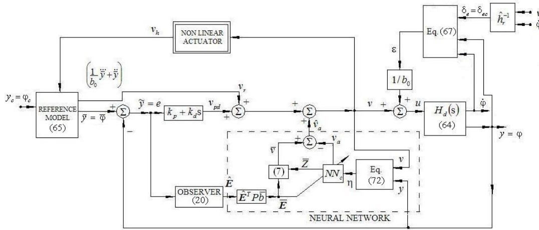
Fig. 6. Block diagram of the system for the control of aircrafts' roll angle
