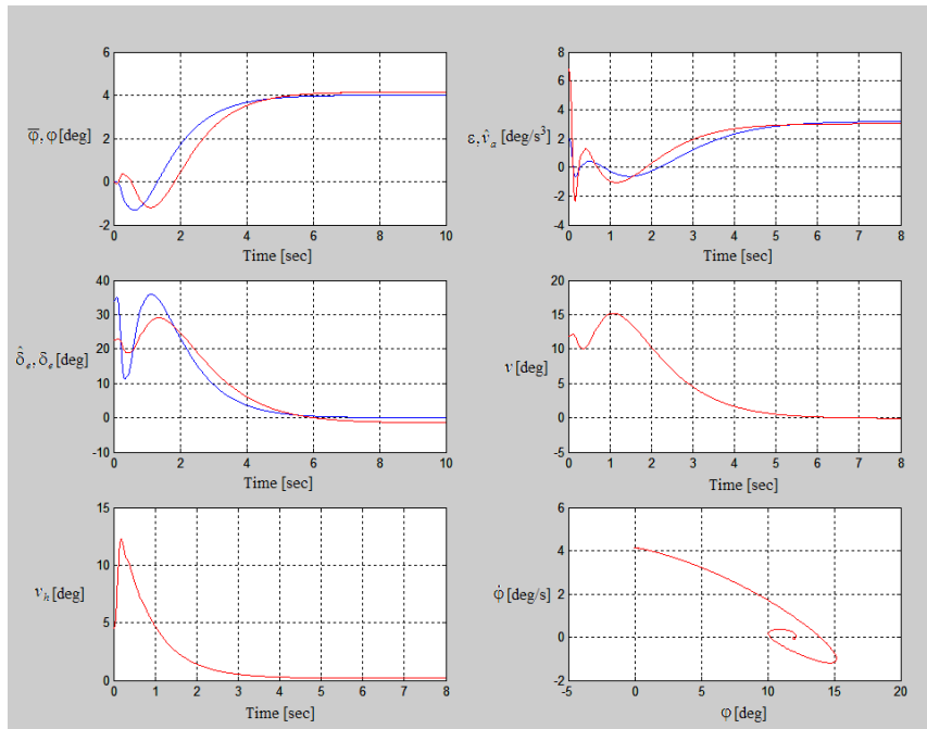
Fig. 14. Time characteristics in the case of non-linear actuator’s use
