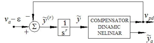
Fig. 4. Block diagram of the dynamic error's model
