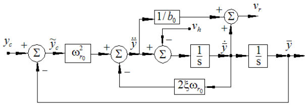
Fig. 7. The block diagram of the reference model
