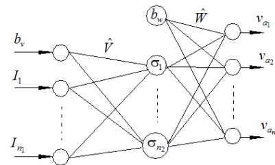
Fig. 2. The neural network
