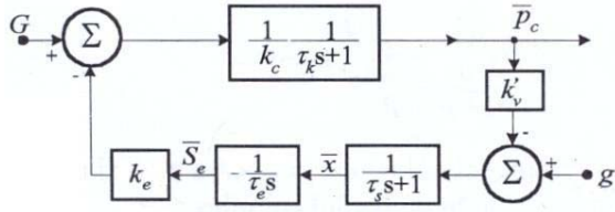
Figure 4: The block diagram of the ARS
